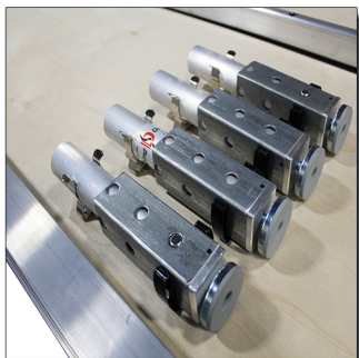
Adjustable height legs mounted to the underside of a stage deck
