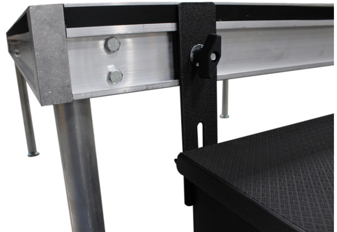
Stair Box attached to Stage Deck
